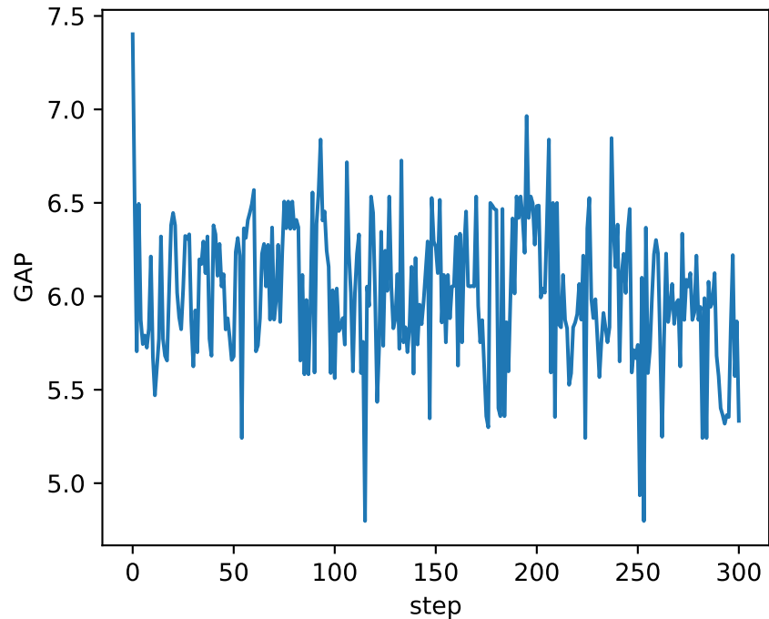
GAP - evolution
