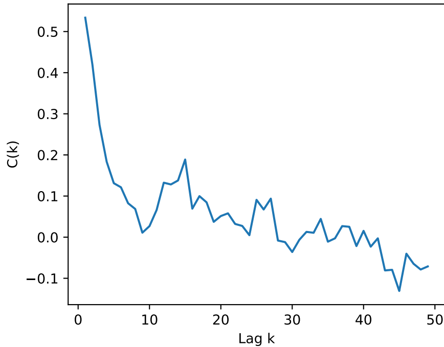
HOMO Autocorrelation
