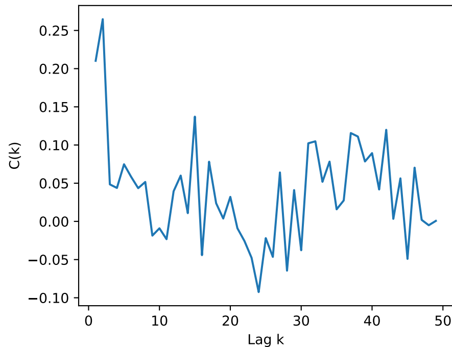
GAP Autocorrelation
